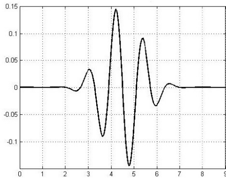
Fig. 2. Wavelet functions of quartic B-spline wavelet
