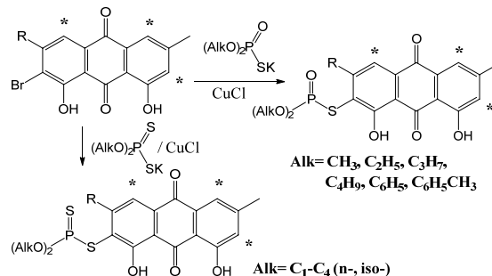
Fig. 6 Thiophosphorylation of chrysophanol
