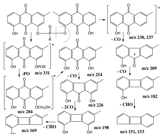
Fig. 5 MS-fragmentation of P-acylic anthraquinones
