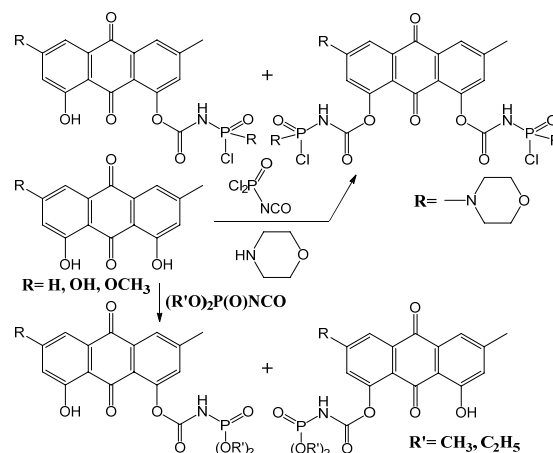
Fig. 8 Isocyanatophosphorylation of anthraquinones
