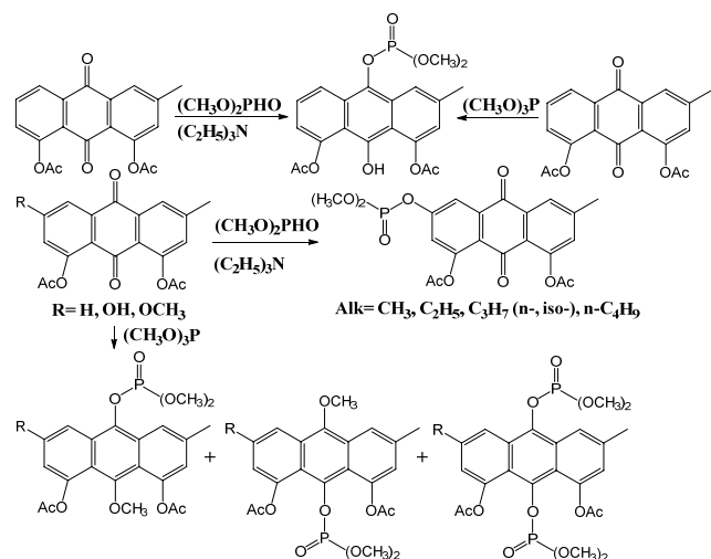
Fig. 9 Alkoxyphosphorylation of anthraquinones
