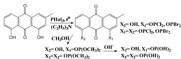
Fig. 2 P-acylation of chrysophanol
