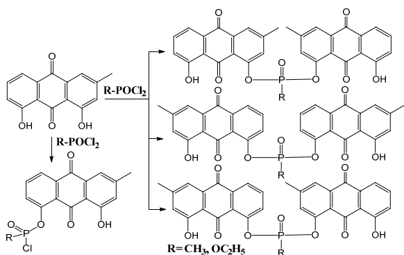
Fig. 4 P-acylic dimerization of chrysophanol
