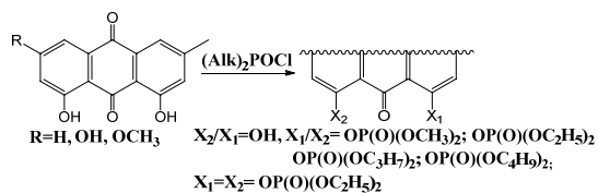
Fig. 3 Chloroanhydride P-acylation of anthraquinones
