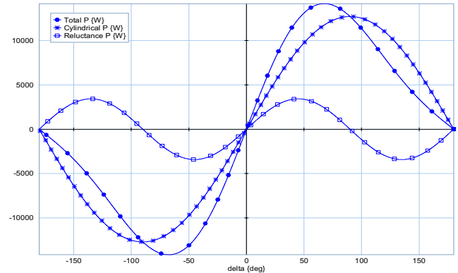
Fig. 14 Real power-angle curves in salient-pole synchronous generator
