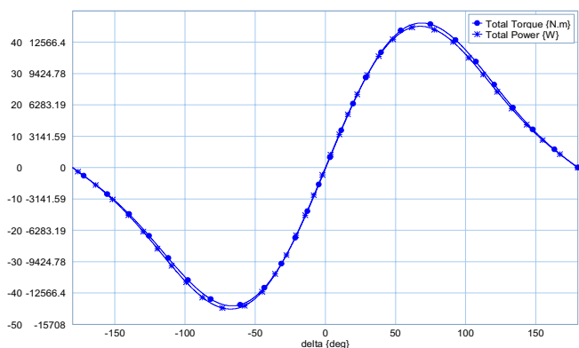
Fig. 16 Torque-angle curve
