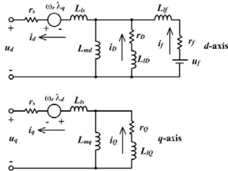
Fig. 1 d -axis and q -axis electrical equivalent circuit
