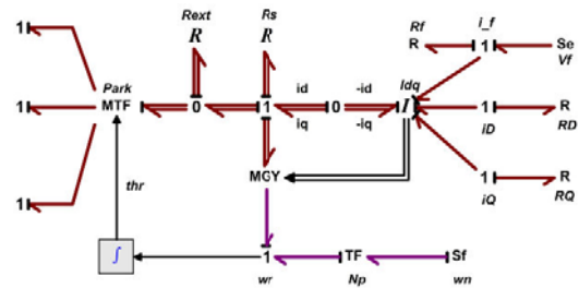
Fig. 6 Synchronous generator vector bond graph
