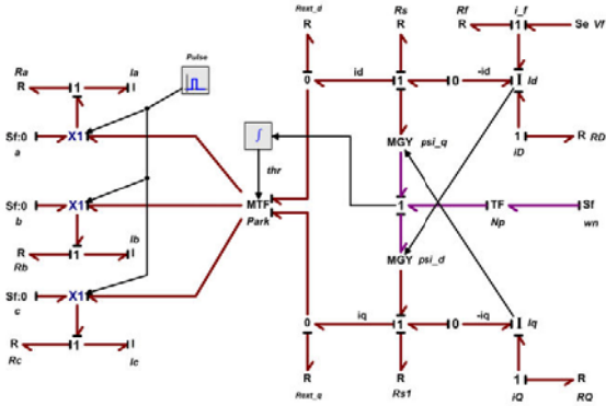
Fig. 3 Sudden short-circuit test in bond graphs
