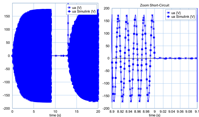
Fig. 4 Stator voltage at phase-a
