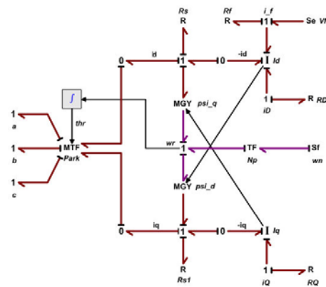
Fig. 2 Bond graph model of synchronous generator
