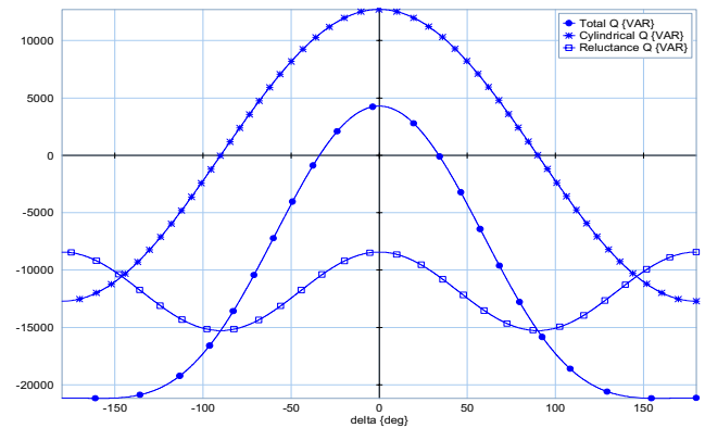
Fig. 15 Reactive power-angle curves in salient-pole synchronous generator
