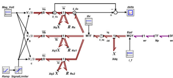
Fig. 13 Phasor bond graph with variable angle load
