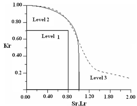
Fig. 1 FAD three levels of investigation
