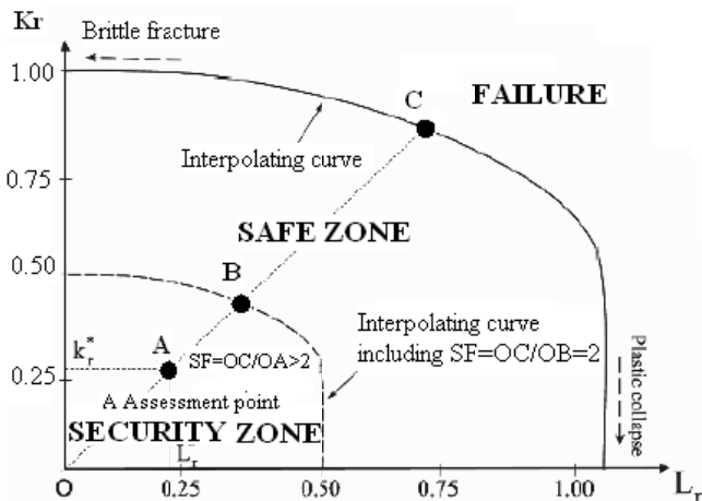
Fig. 4 Calculation of the safety factor
