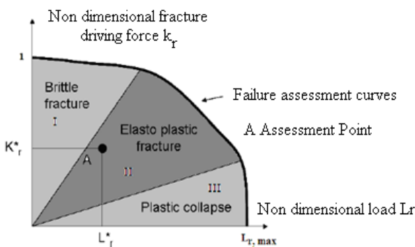
Fig. 2 Domain failure assessment diagram
