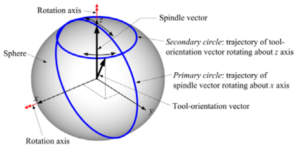
Fig. 1 Illustration of the spherical two-circle method
