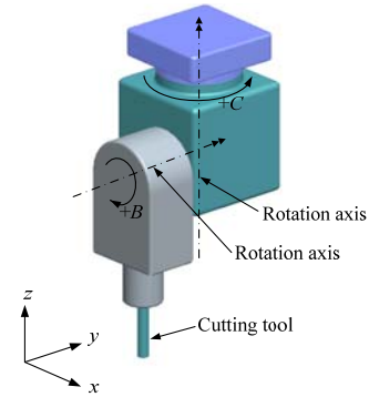
Fig. 2 Rotation mechanism of a spindle-tilting machine
