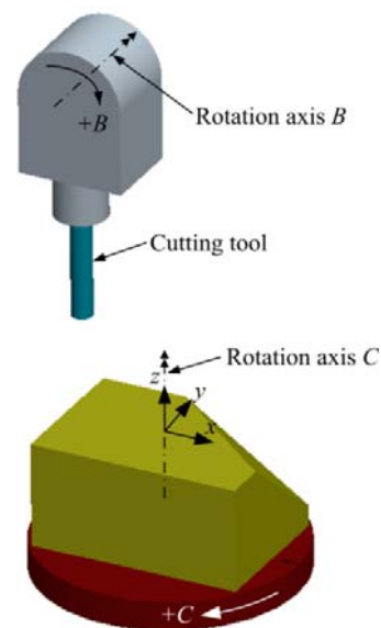
Fig. 4 Rotation mechanism of a hybrid-type machine
