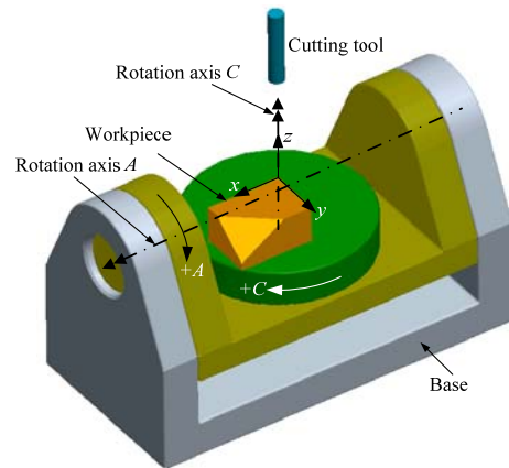
Fig. 3 Rotation mechanism of a table-tilting machine
