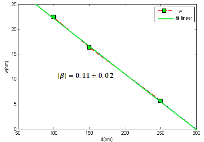
Fig. 4 ZnO layer roughness based on thickness of curve slope, it equals growth rate ( \beta )
