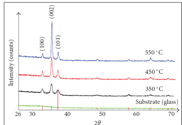
Fig. 7 The XRD pattern of ZnO thin film on glass (annealed at 350°C, 450°C, and 550°C)
