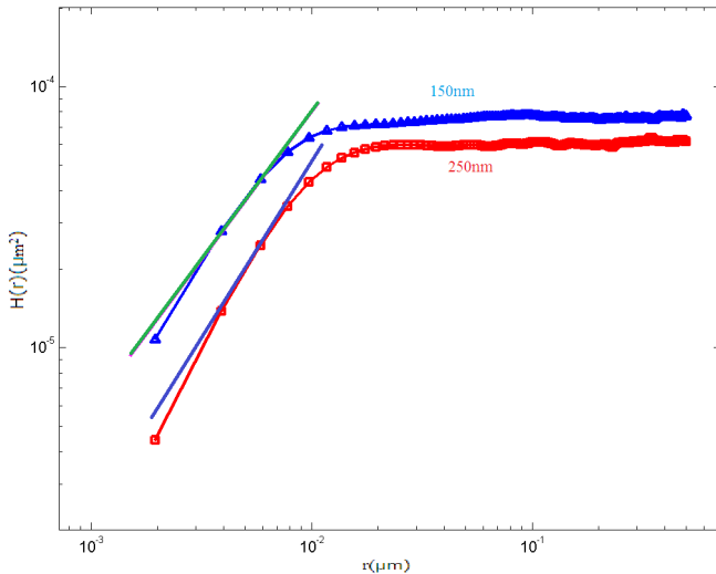
Fig. 3 The height-height correlation function H(r) based on r with thickness of 150 nm and 250 nm
