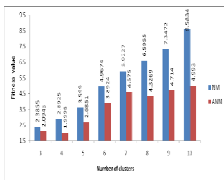
Fig. 8 Experiment results for RPBM data
