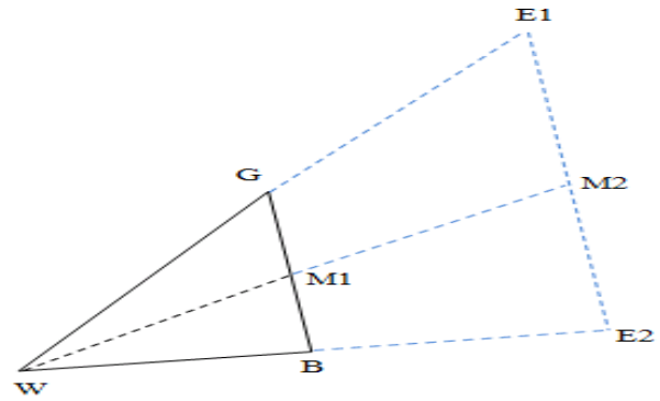
Fig. 6 Finding spread out point and its midpoint
