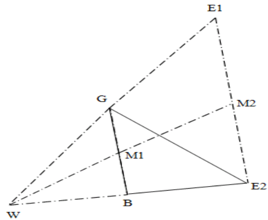
Fig. 7 Finding new triangle with available best points
