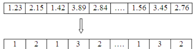
Fig. 5 The representation of vertex for clustering
