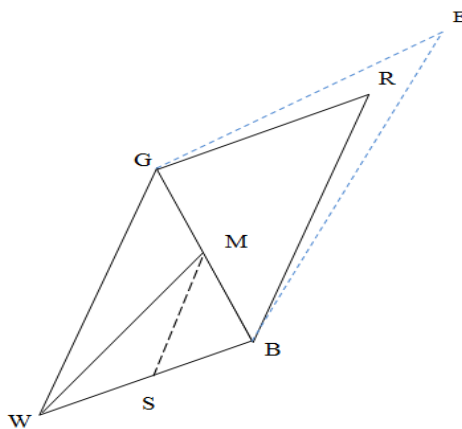
Fig. 2 Operations performed on initial triangle
