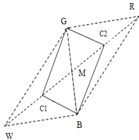
Fig. 3 Finding contraction points
