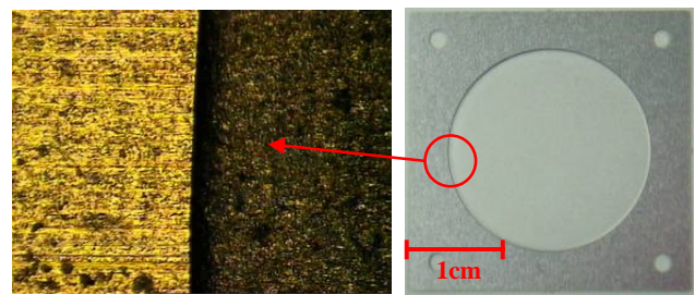
Fig. 4 The fabricated stainless steel chamber layer
