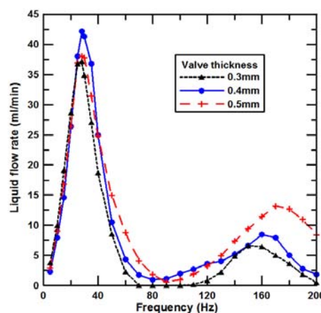
Fig. 11 Measured water flow rate versus operating frequency for three different check valve thicknesses
