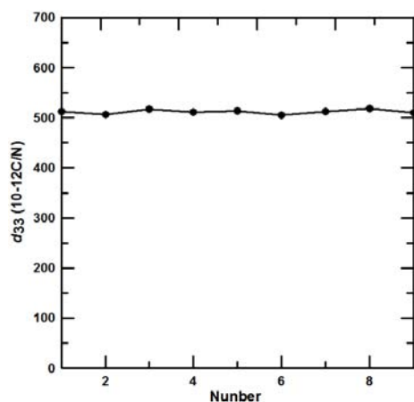
Fig. 6 d_{33} characteristics of the piezoelectric disc
