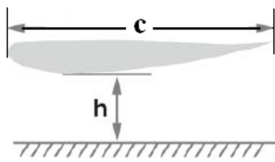
Fig. 2 Physical model of a race car wing
