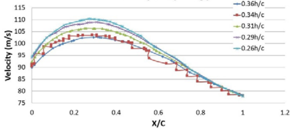
(g) Velocity variations at 17° angle of attack
