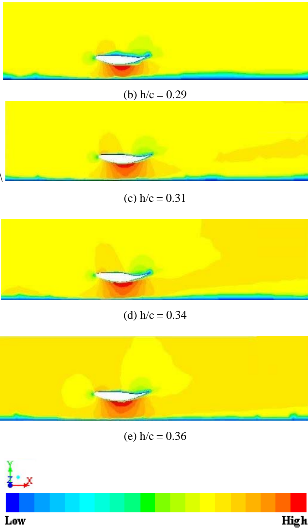
Fig. 5 (a)-(e) Velocity contours at different ground clearance ( h/c ) at zero angle of attack
