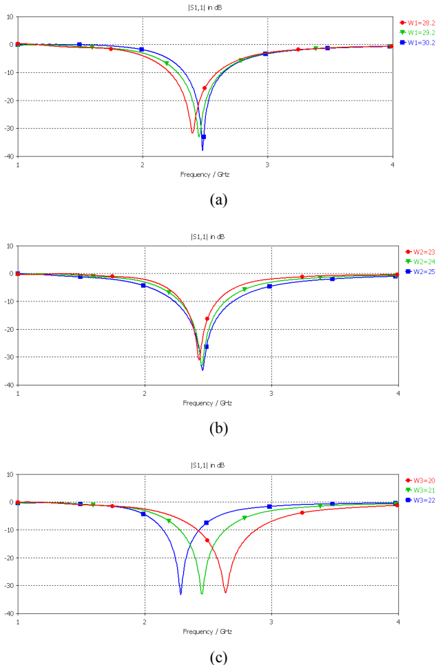
Fig. 4 Simulated return loss of AMC for varied value of W_1 , W_2 , and W_3
