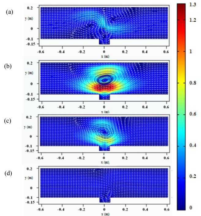
Fig. 4 Swirling flow of ground wire in various \theta : (a) \theta = 0^\circ (b) \theta = 60^\circ (c) \theta = 120^\circ and (d) \theta = 180^\circ when consider within a channel flow and u_i = 0.1 m/s
