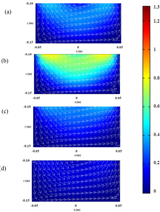
Fig. 5 Airflow of ground wire in various \theta : (a) \theta = 0^\circ (b) \theta = 60^\circ (c) \theta = 120^\circ and (d) \theta = 180^\circ when consider within a channel flow and u_i = 0.1 m/s
