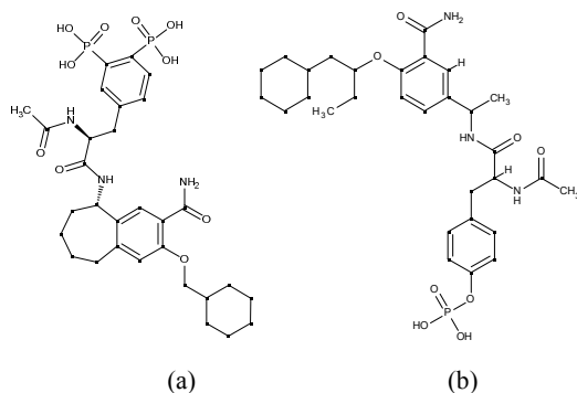
Fig. 1 Chemical structures of (a) AP22408 and (b) CID 67698995
