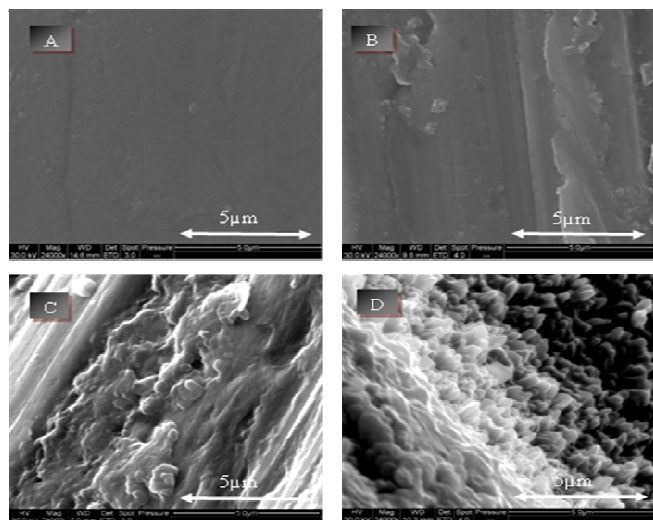
Fig. 1 SEM images of the FeCrAlloy wires before and after the physical pre-treated (A) as supplied, (B) sand-papered, (C) acid and base washed and (D) oxidised at 1000^\circ\text{C} for 4 h
