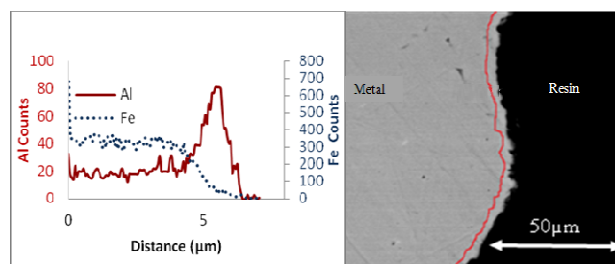
Fig. 4 Elemental line scans across the wires oxidised at 1000^\circ\text{C} , 4h (for clarity, the red line approximates the position of oxide layer)
