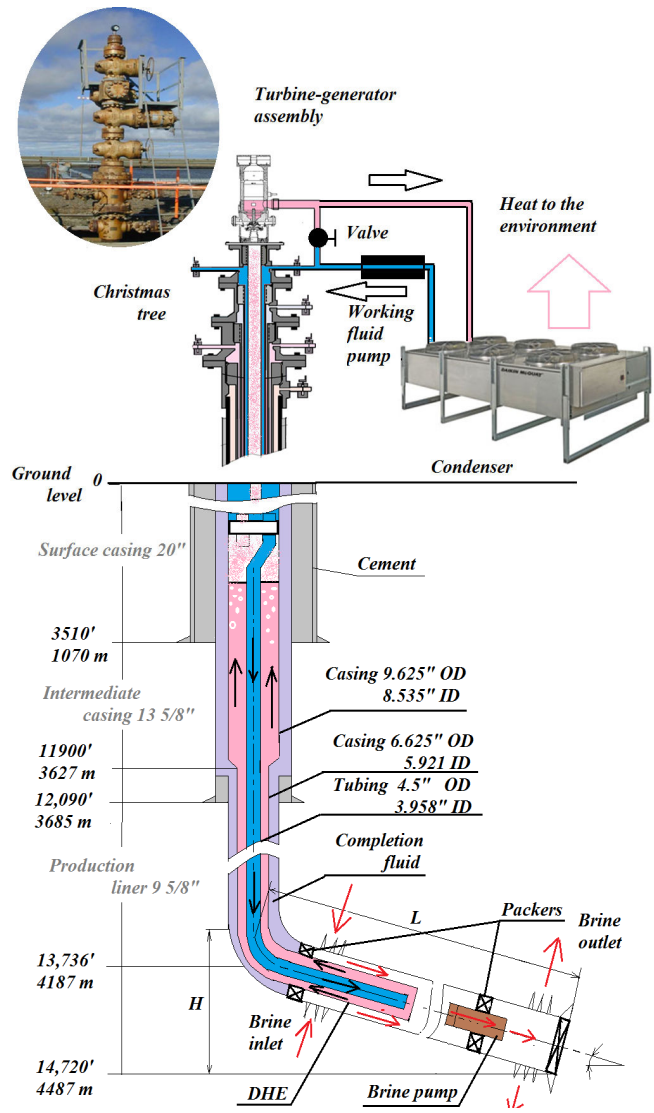
Fig. 2 Single well power unit schematic design
