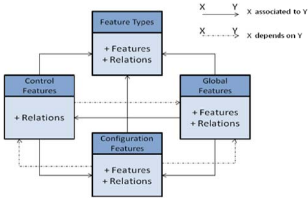
Fig. 2 Meta-features connections
