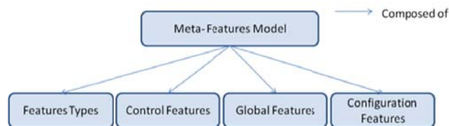
Fig. 1 Meta-features Model
