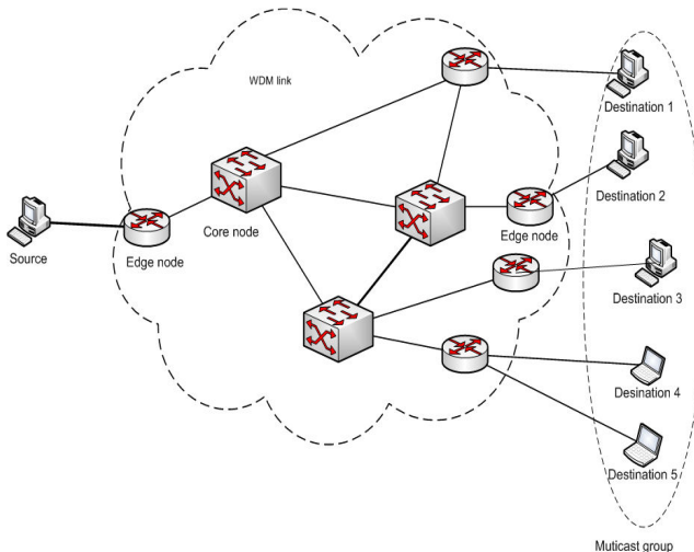
Fig. 1 Multicasting concept
