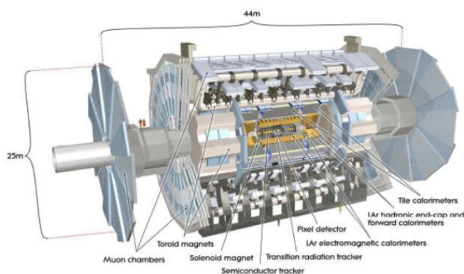
Fig. 3 ATLAS experiment
