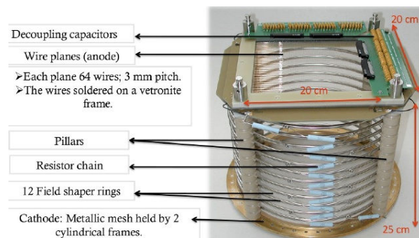
Fig. 4 Inner part of the LAr
