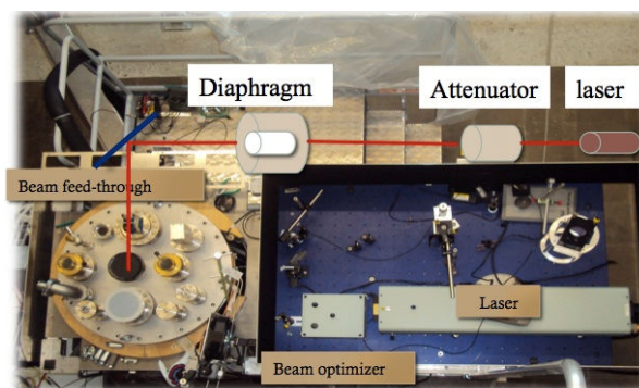
Fig. 6 Experimental setup of the laser beam
