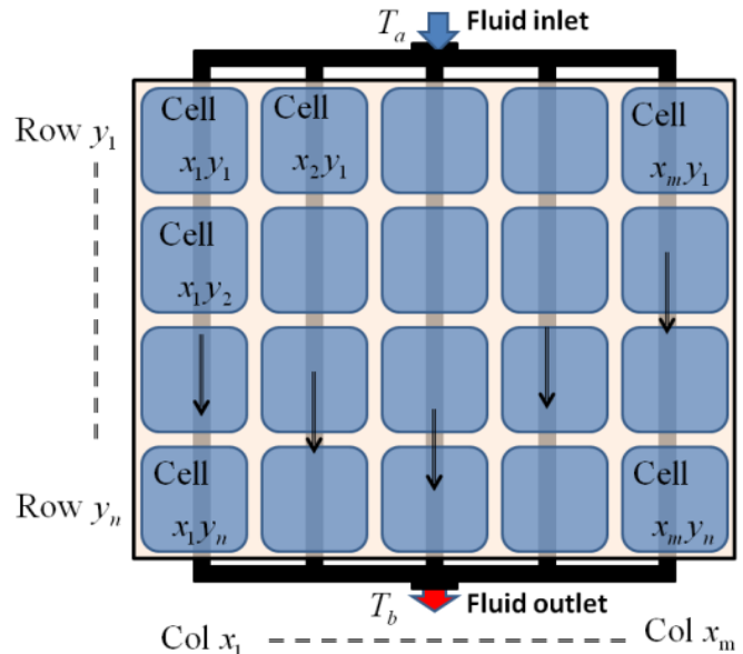
Fig. 3 Example design of a PV panel consisting of N series-connected solar cells
