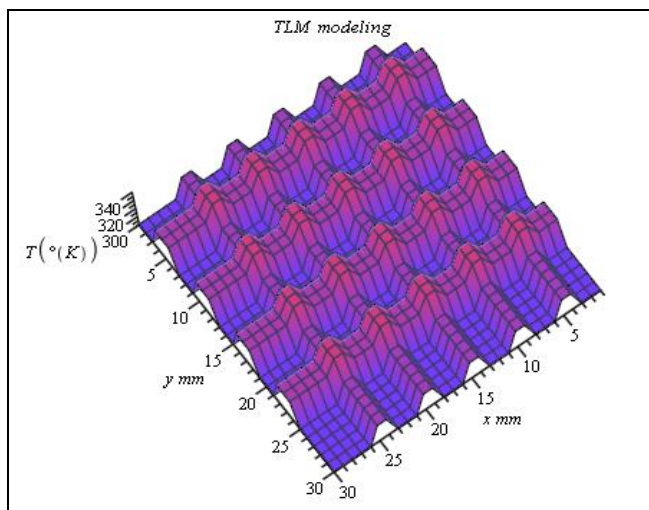
Fig. 4 Temperature distributions on poly-Si cell
