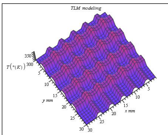
Fig. 5 Front face temperature distributions for the a i Si cell
