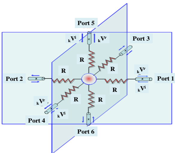
Fig. 1 Equivalent TLM of a node
