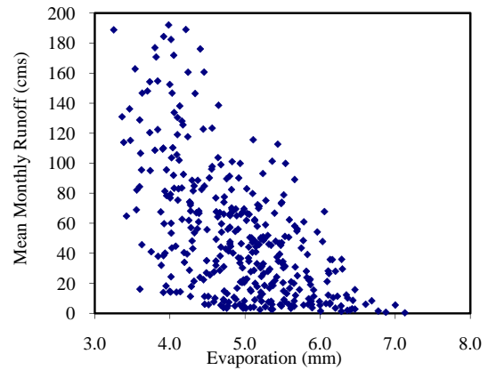
Fig. 6 The relationship between mean monthly runoff and mean monthly evaporation
