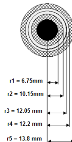
Fig. 5 Cable Configuration
