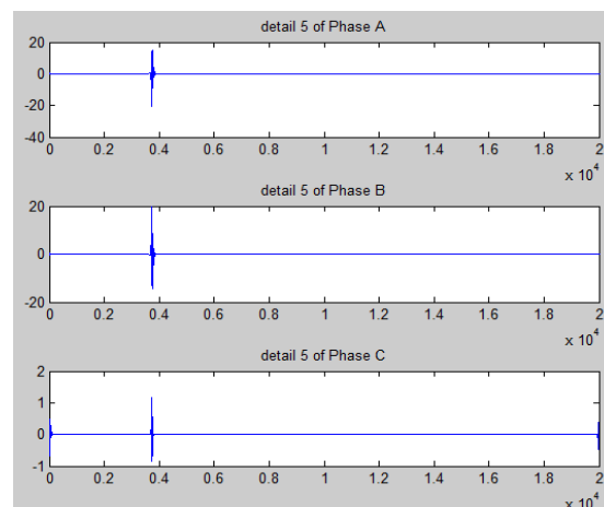
Fig. 3 Detailed coefficients of Line to Line Fault case
