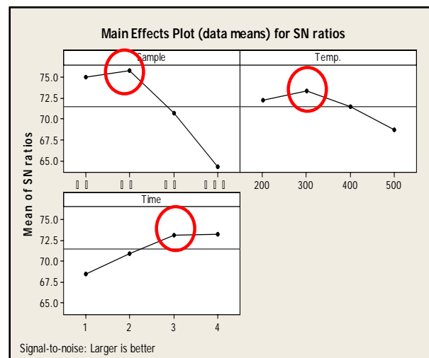
Fig. 1 S/N ratios of different operation parameters
