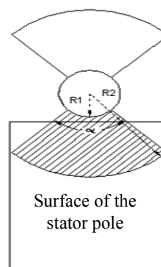
Fig. 8 The effective area crossed magnetic flux
