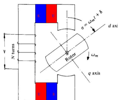
Fig. 1 Simple reluctance generator
