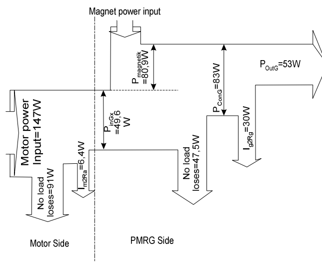
Fig. 18 Power flow scheme
