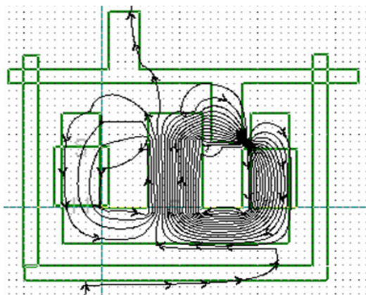
Fig. 12 The mapping of magnetic flux
