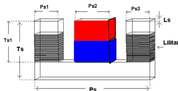
Fig. 10 Specifications stator P_s = 15.2 \text{ cm} , T_s = 10.1 \text{ cm} , L_s = 6.3 \text{ cm} , P_{s1} = P_{s3} = 2.5 \text{ cm} , P_{s2} = 5 \text{ cm} , T_{s1} = 7.6 \text{ cm} , Number of winding = 530 turn, Size of copper = 0.5 mm
