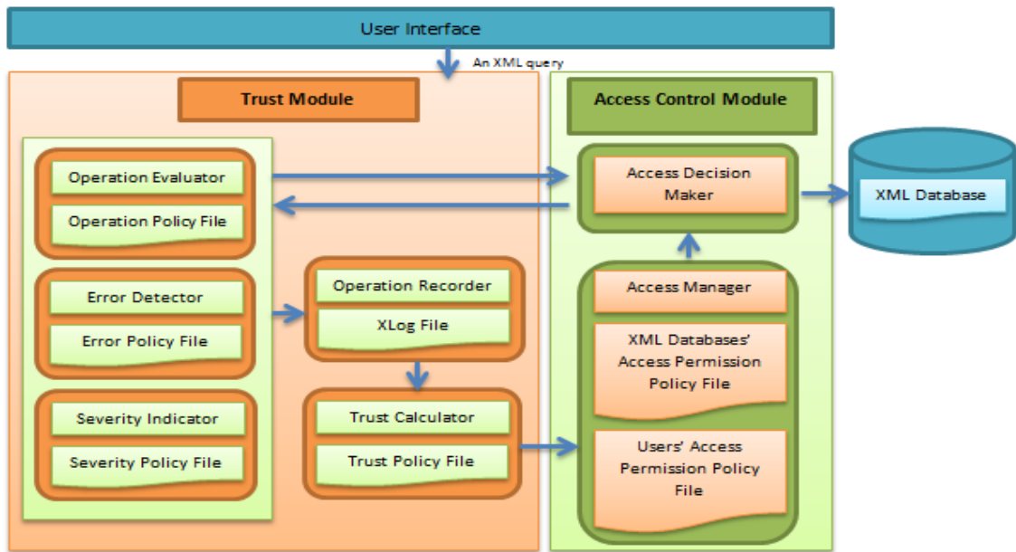
Fig. 1 XTrust Architecture
