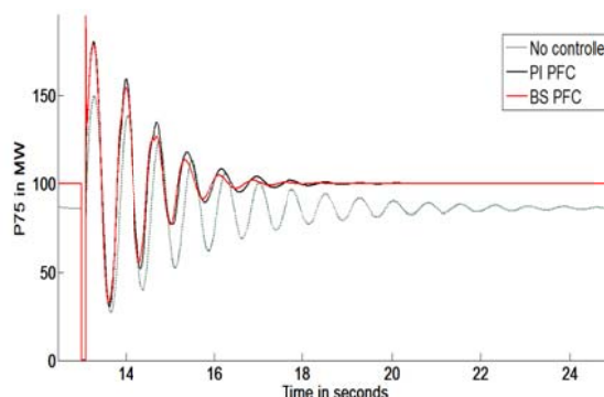
Fig. 8 Oscillations in Power through the line 7-5 for Three-Phase Short Circuit at Bus-7
