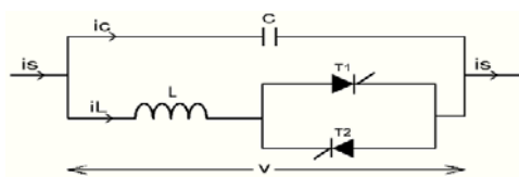
Fig. 2 Configuration of a TCSC
