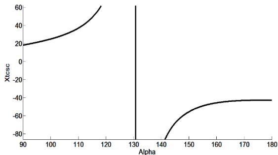
Fig. 5 X_{TCSC} vs. \alpha Characteristic of TCSC
