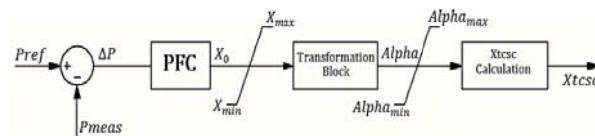
Fig. 3 Power Flow Controller (PFC) diagram for TCSC
