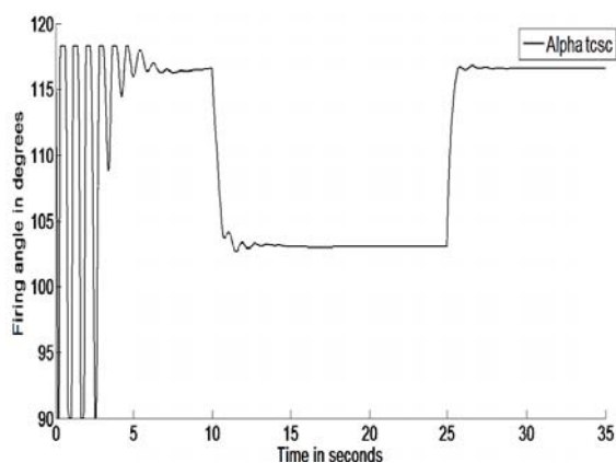
Fig. 7 (c) TCSC Firing Angle
