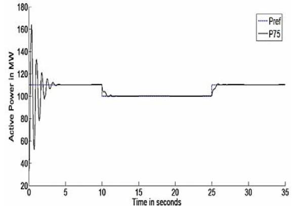
Fig. 6 (a) Power Flow in line 7-5
