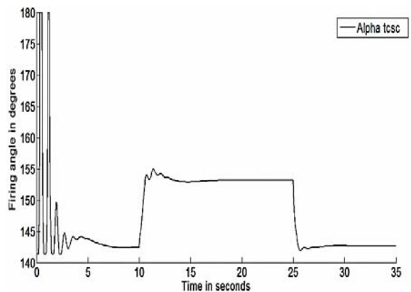
Fig. 6 (c) TCSC Firing Angle
