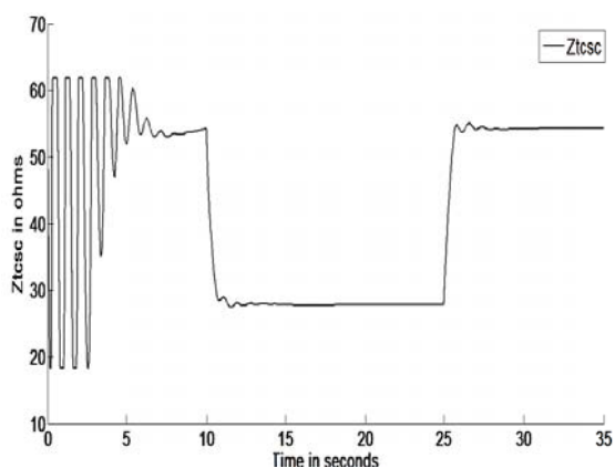
Fig. 7 (b) X_{TCSC} of TCSC
