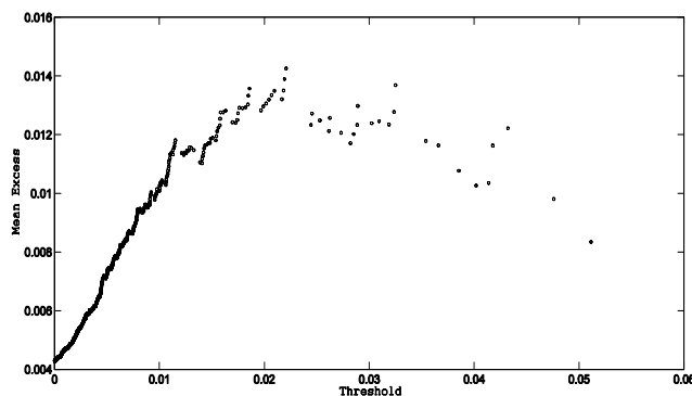
Fig. 3 Mean Excess Plot for SEMDEX losses
