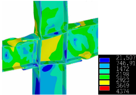
(a) Von-Mises stress distributions for analytical model U1-FUW1 based on experiments[20]
