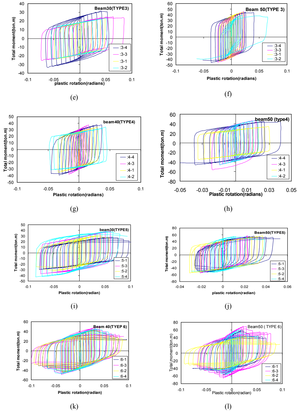
Fig. 4 Cyclic response of analytical models
