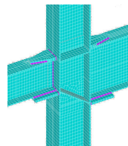
(a) Inclined continuity plate (Y=1)
