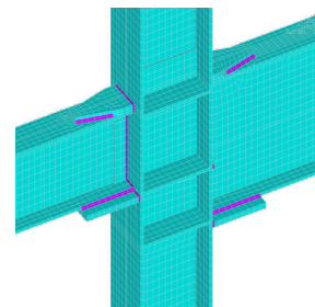
(b) Straight continuity plate (Y=2)
