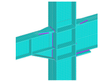
(c) One sided haunch connection (Y=3)
