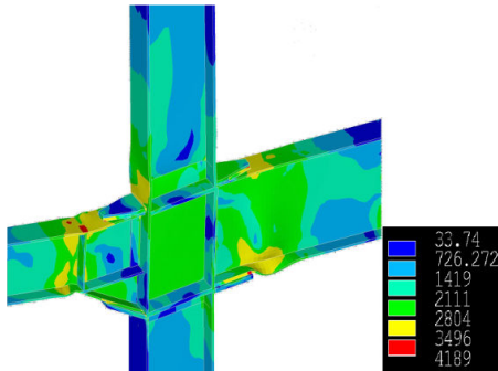
(b) Von- Mises stress distributions for analytical model U1-FUW3 based on the experiments[20]
