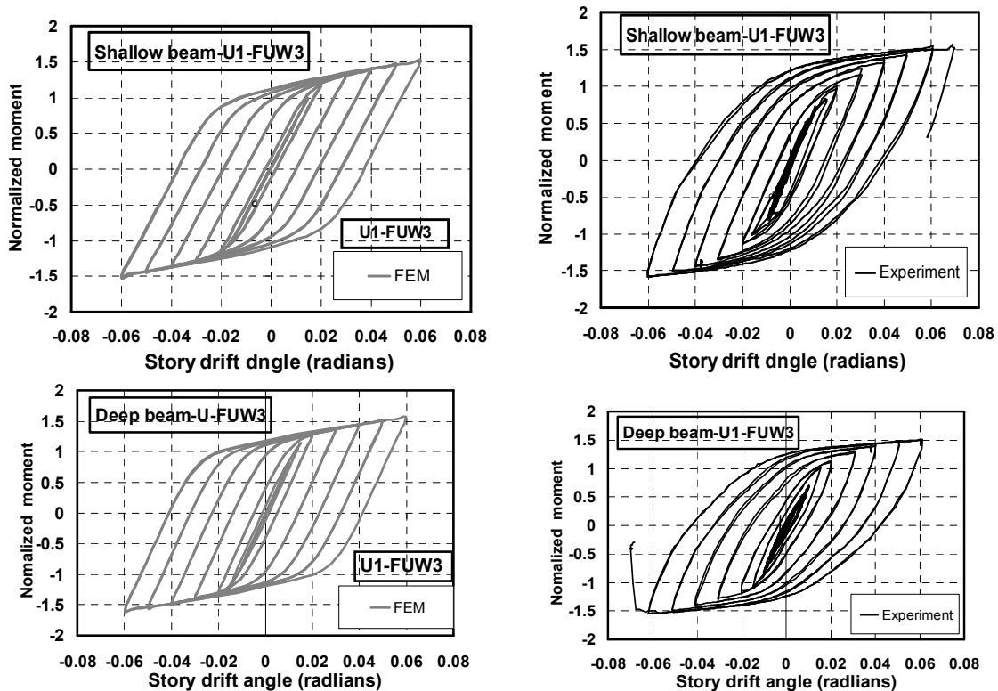
Fig. 1 Experimental and analytical model for the deep and shallow beams for test specimens U1-FUW3
