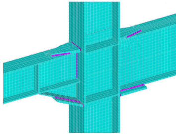
(d) One sided haunch with inclined cover plate (Y=4)
