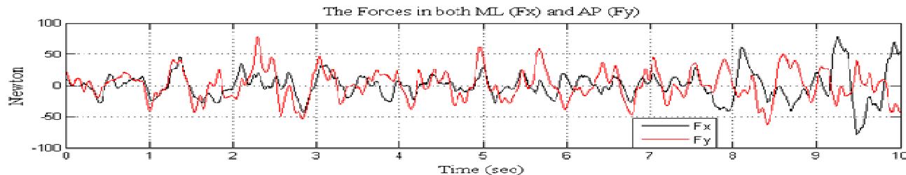
Fig. 9 The applied forces in both the F_{ML} and F_{AP} directions in static balance (Romberg 2-foot flat) and (Romberg 1-foot-tiptoes) (Units = N)
