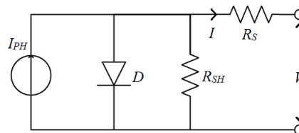
Fig. 1 Equivalent circuit of solar photovoltaic cell
