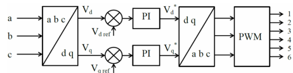
Fig. 2 Voltage regulator for solar PV
