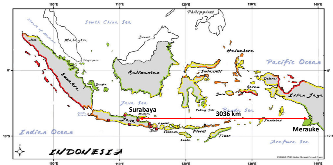
Fig. 8 Locations of HF Channel Measurement Systems
