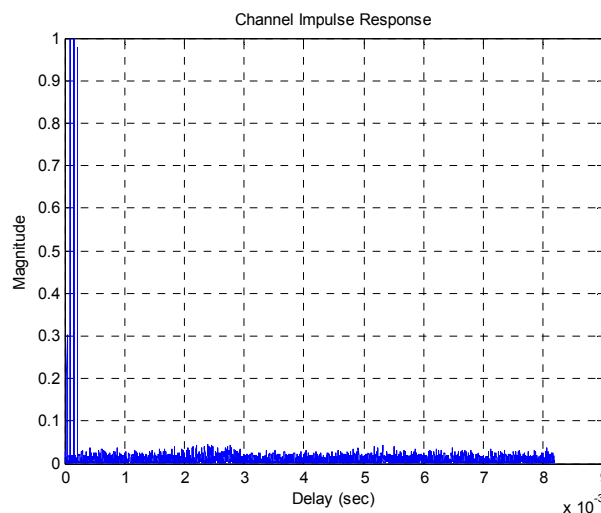
Fig. 5 Channel Impulse Response
