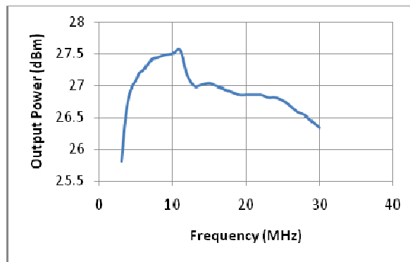
Fig. 6 Frequency Response of Amplifier 1
