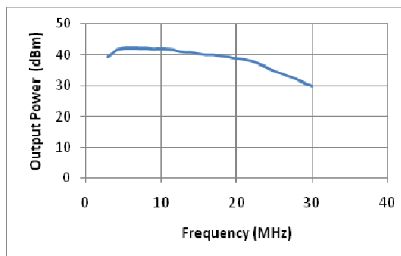
Fig. 7 Frequency Response of Amplifier
