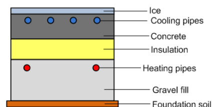
Fig. 1 A typical ice pad structure
