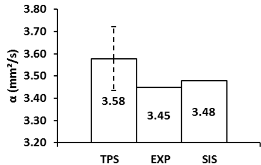
(b) Thermal diffusivity
