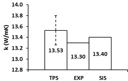
(a) Thermal conductivity
