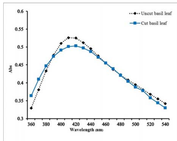
Fig. 4 UV-Vis spectra of silver nanoparticle received from uncut basil leaf (A) and cut basil leaf (B)
