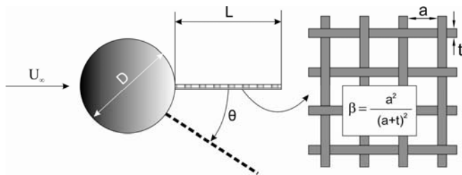
Fig. 1 Schematic presentation of the control technique and definition of porosity, \beta of permeable plate
