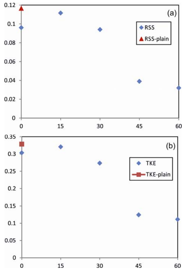
Fig. 5 Maximum values of Reynolds Shear Stress (a) and Turbulent Kinetic Energy (b) for all cases
