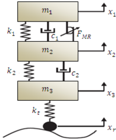
Fig. 2 Quarter car model with MR suspension
