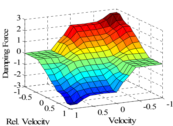
Fig. 6 Forward FLC input/output surface
