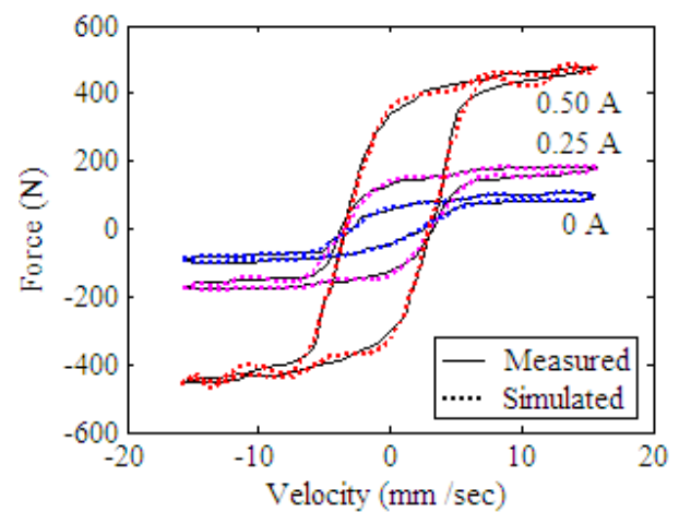
Fig. 1 Experimental and polynomial fitted curves (0.5 Hz, \pm 5 mm): Force vs. Velocity
