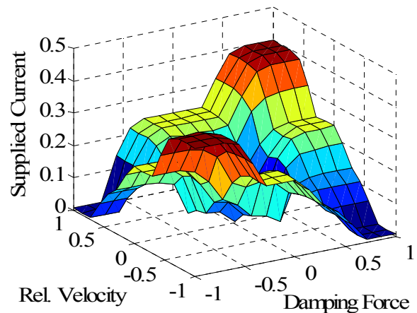
Fig. 7 Inverse FLC input/output surface
