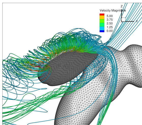
Fig. 4 Three-dimensional stream traces around the leading edge and wing tip regions
