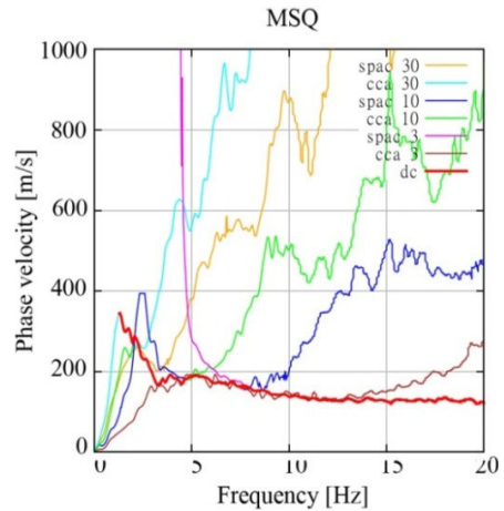
(g) Dispersion curve at MSQ site
