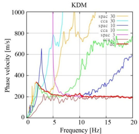
(c) Dispersion curve at KDM site
