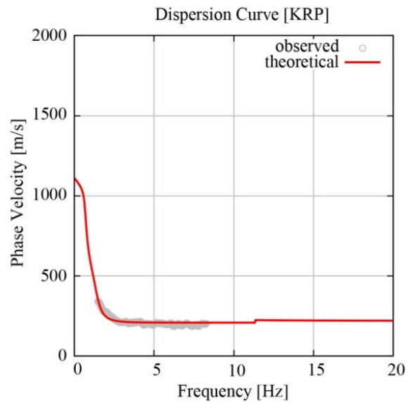
Fig. 13 Dispersion curve at KRP
