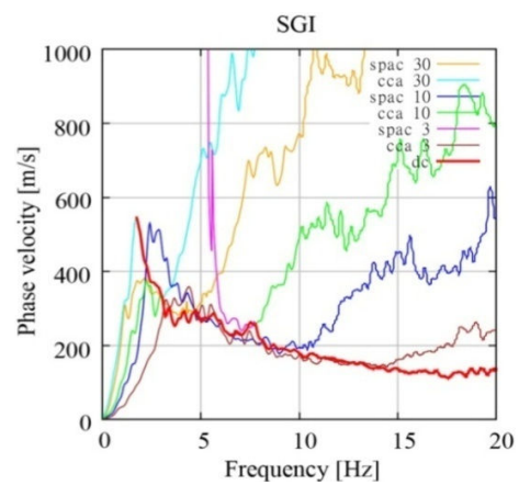
(h) Dispersion curve at SGI site
