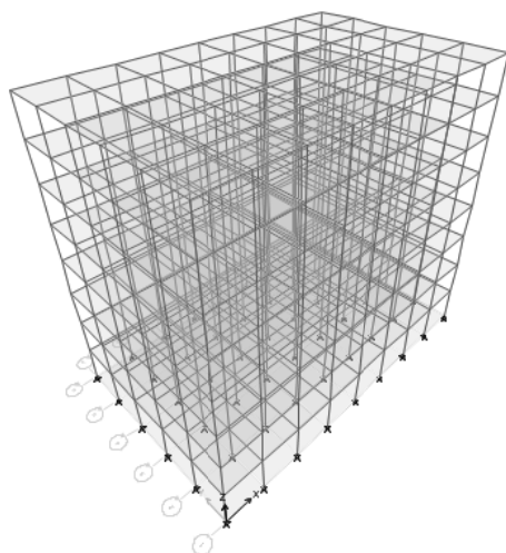
Fig. 2 3-D view of building
