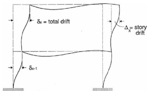
Fig. 15 Deflection of frame structure
