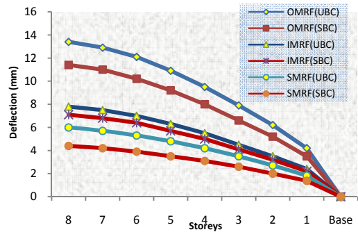
Fig. 10 Story displacement in long-dir for Jazan
