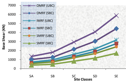
Fig. 3 Base Shear for Yanbu
