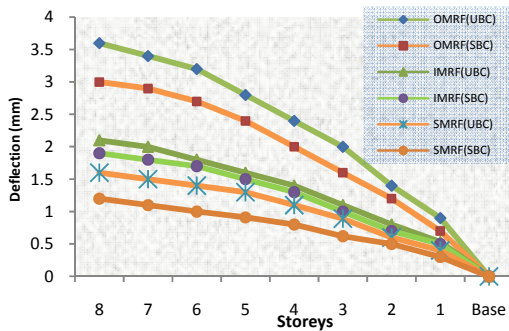
Fig. 7 Story displacement in short-dir for Yanbu
