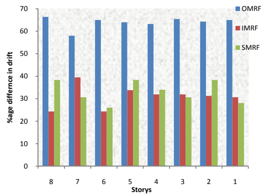
Fig. 12 %age difference in drift for Yanbu (long dir.)
