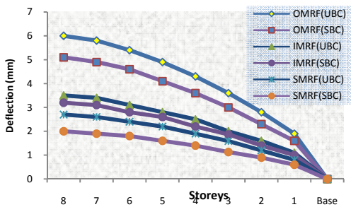
Fig. 8 Story displacement in long-dir for Yanbu
