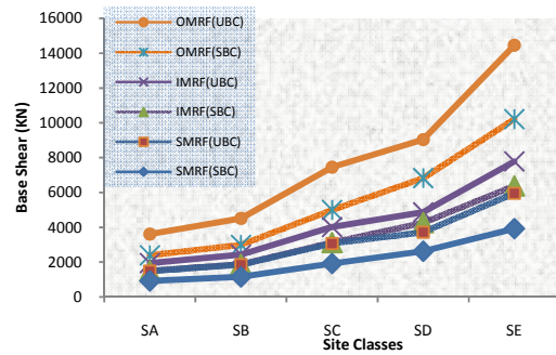
Fig. 4 Base Shear for Jazan
