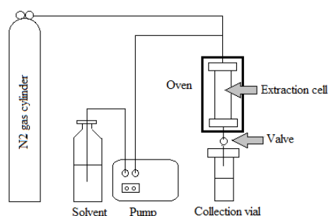
Fig. 2 Schematic diagram of ASE 350
