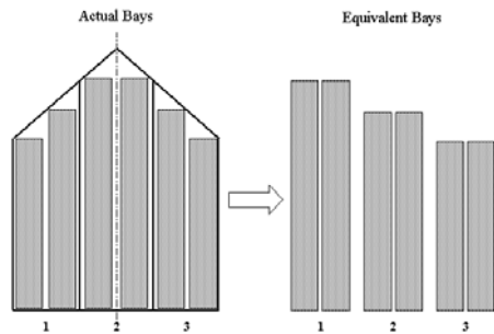
Fig. 4 Converting Seating Areas into Equivalent Bays [1]
