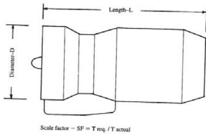
Fig. 5 Rubber Scaling of an Engine [3]
