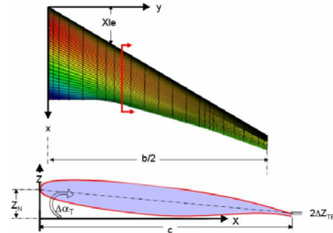
Fig. 9 Parameters used in 3D Wing CST Derivation [10]
