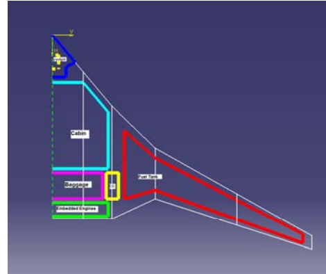
Fig. 8 Implemented Internal Arrangement of Major Components in the Semi-span of a BWB Aircraft
