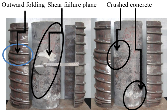
(e) Failure modes of concrete core of confined UHSCFST columns (CS(8)10-4-139-120)
