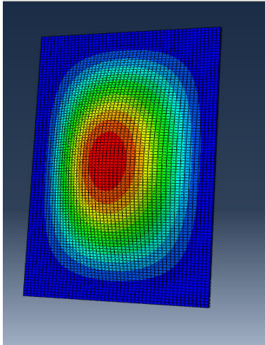
Fig. 12 Sixth Modes shape U_{max}=1mm , f_0=26.501 HZ
