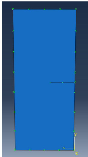
Fig. 13 Crack initiation in plate composite
