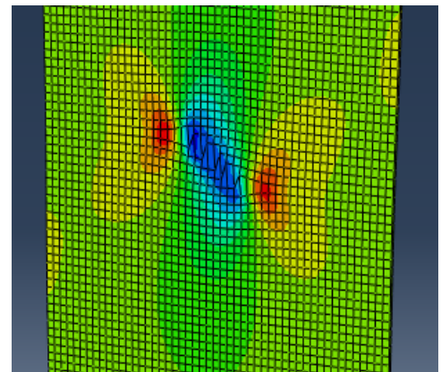
Fig. 19 Crack inclined angle 30°
