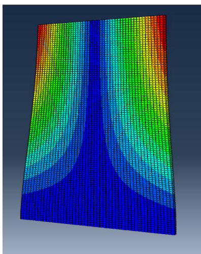
Fig. 8 Second Mode shape torque U_{\max}= 1\text{mm} , f_2=6.0403\text{HZ}
