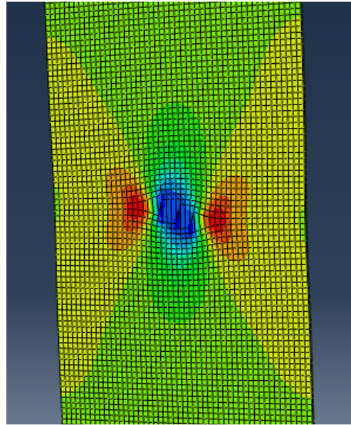
Fig. 18 Crack inclined angle 15°
