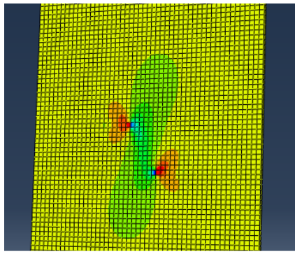
Fig. 21 Crack inclined angle 60^\circ
