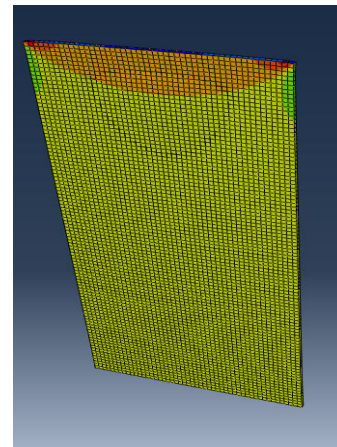
Fig. 5 Maximum strain E_{\max}=4.829 \text{ e}-03
