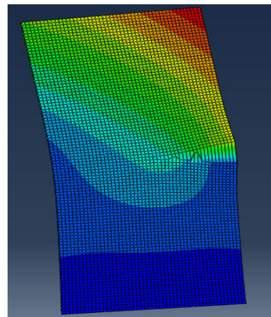
Fig. 16 Maximum displacement by XFEM method U_{max} = 3.088 e-01mm
