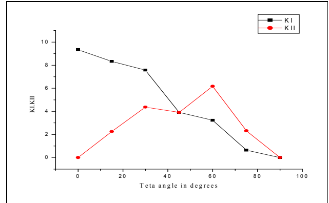
Fig. 24 KI and KII based on the driven plate and an inclined crack centered
