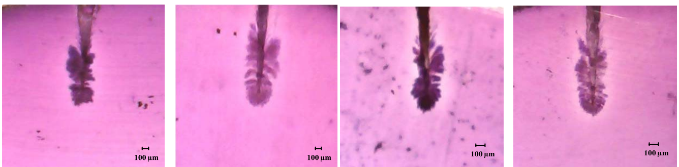
Fig. 6 Water treeing occurrence from CuSO_4 solution
