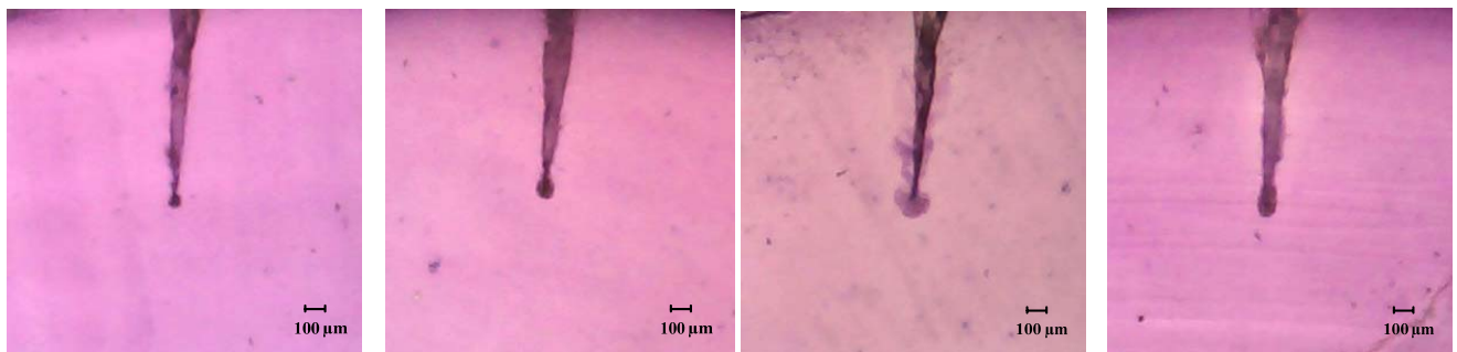
Fig. 7 Water treeing occurrence from FeSO_4 solution
