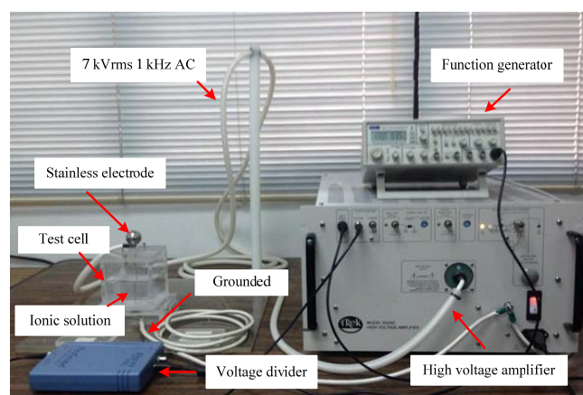
Fig. 4 Experimental setup
