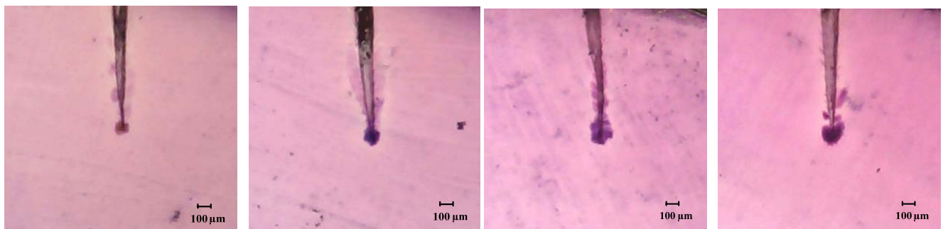
Fig. 8 Water treeing occurrence from K_2SO_4 solution
