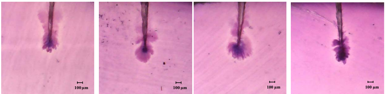
Fig. 5 Water treeing occurrence from Na_2SO_4 solution
