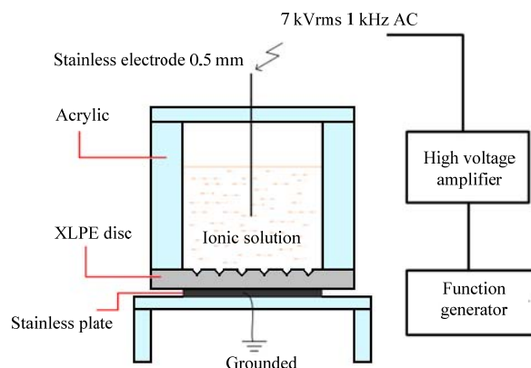
Fig. 3 Schematic diagram of test cell
