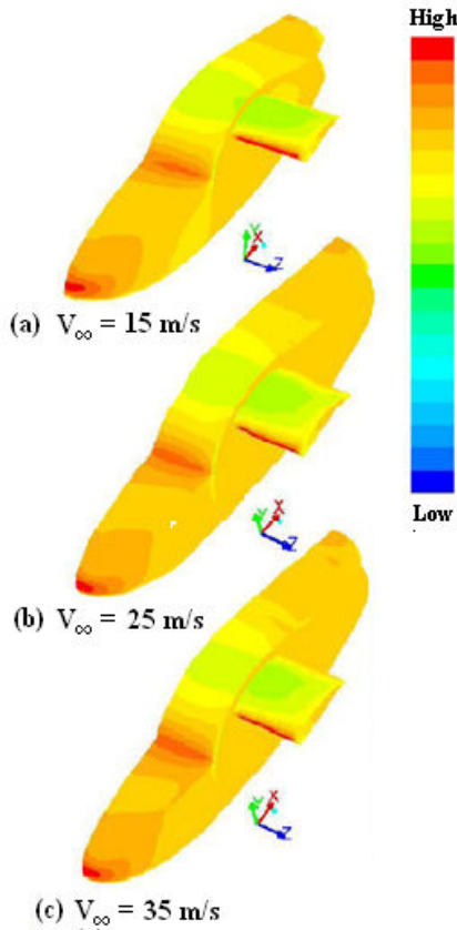
Fig. 12 (a)-(c) Contours of the static pressure at various speeds of Ferrari F430 flying car with short high wing model
