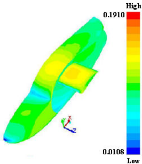
Fig. 13 Contours of Mach number at a free stream velocity of 35 m/s of Ferrari F430 flying car with short high wing model
