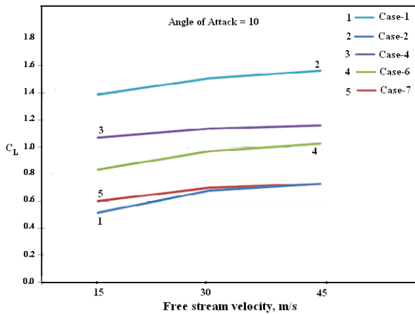
Fig. 17 Comparison of C_L variations for different flying car models at different velocities at an angle of attack of ten
