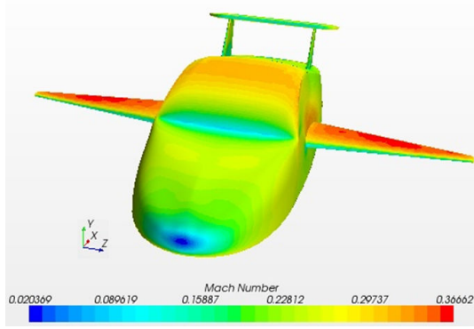
(b) Mach number contours of Ferrari F430 flying car
