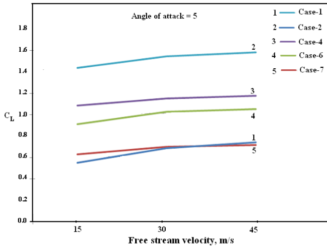
Fig. 16 Comparison of C_L variations for different flying car models at different velocities at an angle of attack of five
