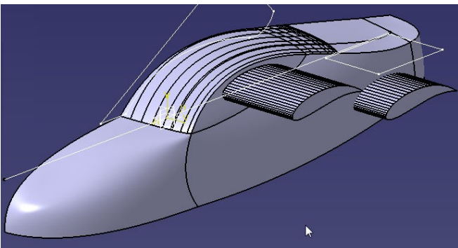
Fig. 6 Ferrari F430 flying car having both high and rear end wings (Case-4)
