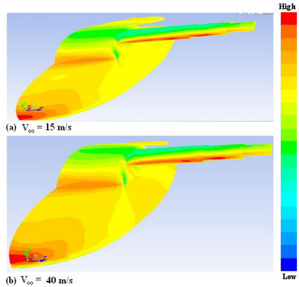
Fig. 14 (a)-(b) Contours of the static pressure at two different speeds of Ferrari F430 flying car with long (extendable) high wings
