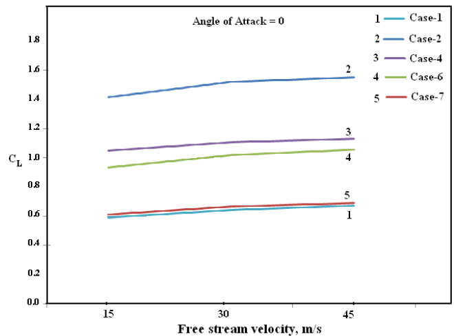
Fig. 15 Comparison of C_L variations for different flying car models at different velocities at zero angle of attack
