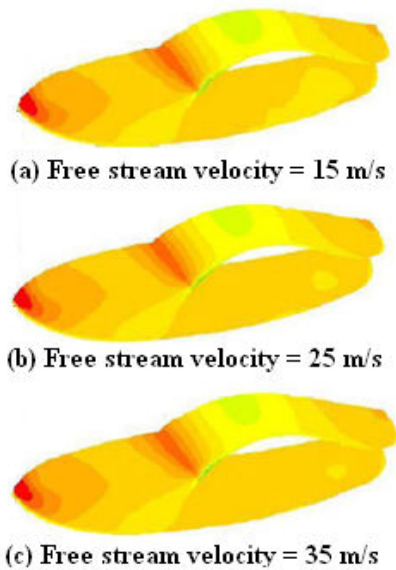
Fig. 10 (a)-(c) Contours of static pressure at various speeds of Ferrari F430 reference car
