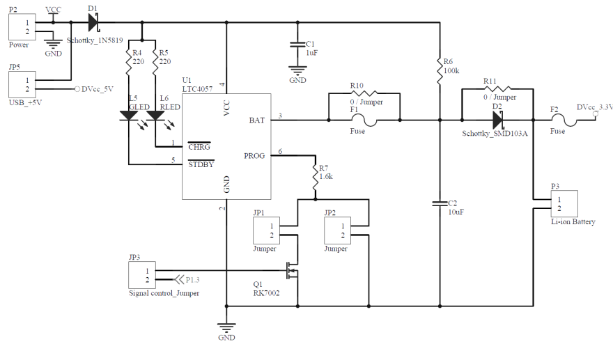
Fig. 3 A simplified representation of the solar-powered battery charger using a TP4057 of schematic
