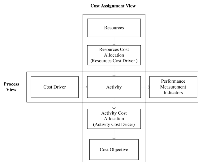
Fig. 2 Two Dimensional Activity-Based Costing Model
