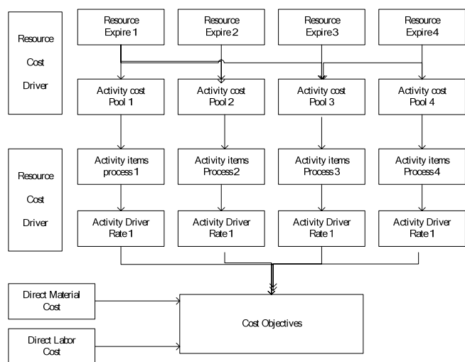
Fig. 1 Two Stage Cost Allocation Flow
