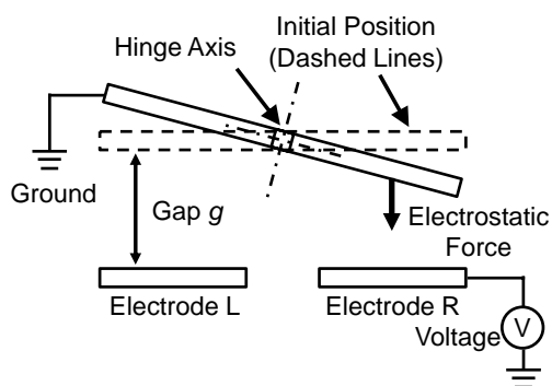
Fig. 2 Drive principle
