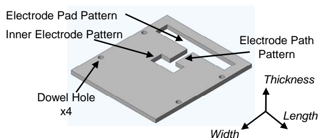
Fig. 4 Designed electrode mask
