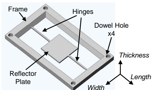
Fig. 3 Designed mirror layer (backside view)
