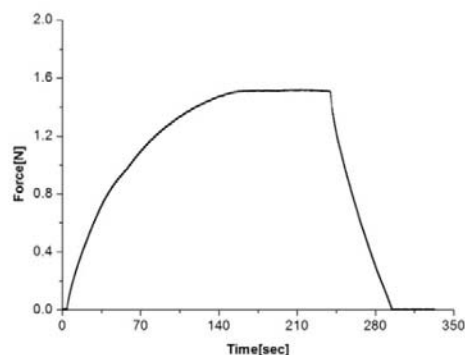
Fig. 3 Blocking force of an IPMC actuator
