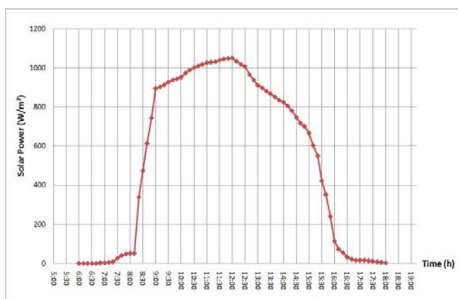
Fig. 4 Graph of solar energy density reflecting on the cell
