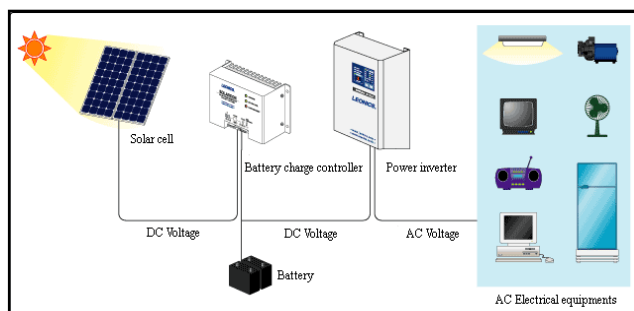
Fig. 1 The diagram of solar generator installed on the roof of the learning center
