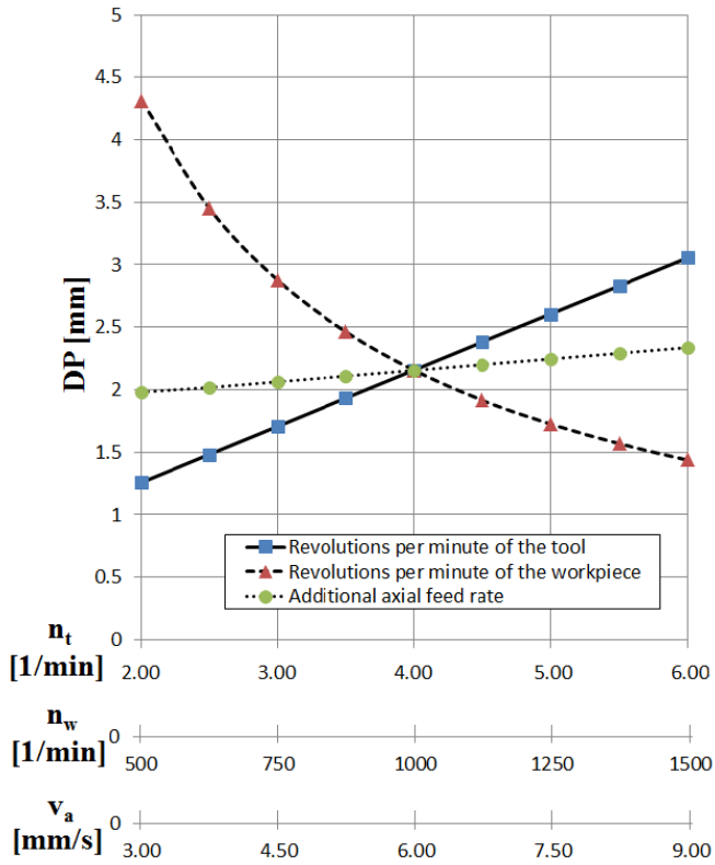
Fig. 5 Effect of the kinematic parameters on the period length of the twist ( DP )
