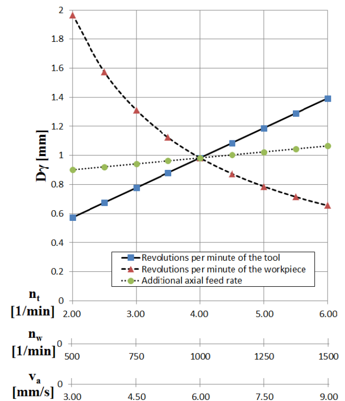
Fig. 4 Effect of the kinematic parameters on the twist angle ( D\gamma )
