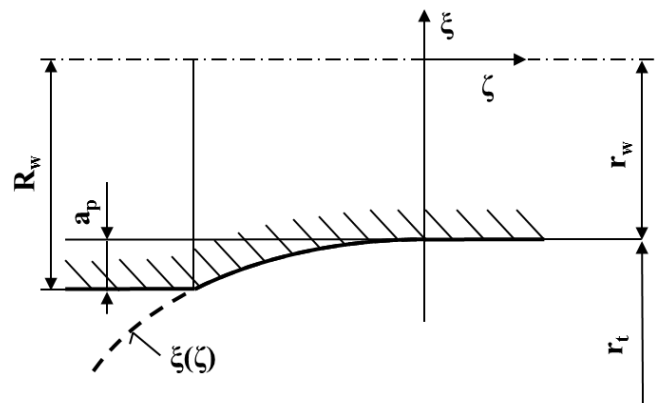
Fig. 3 Illustration of the cut surface equation
