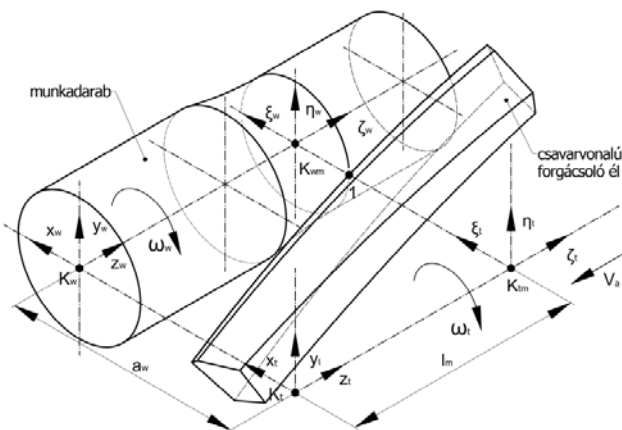
Fig. 2 Kinematical-geometric model of rotational turning, from [17]
