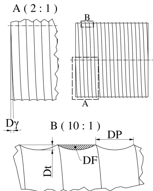
Fig. 1 The parameters of twist measurement
