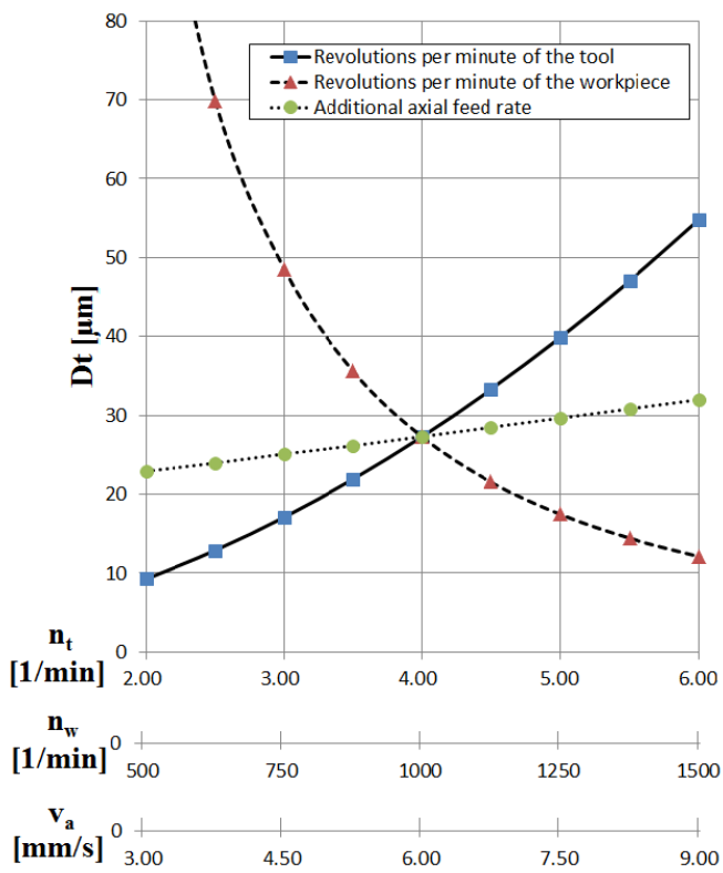
Fig. 6 Effect of the kinematic parameters on the depth of the twist ( Dt )
