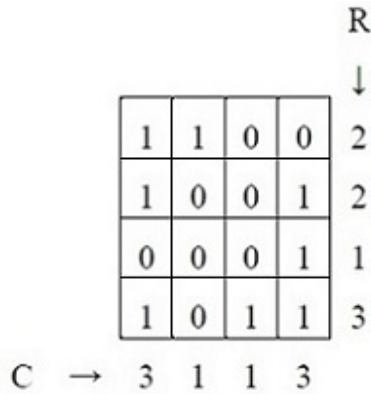
Fig. 2 A 4 × 4 binary matrix and its row projection R = (2,2,1,3) and column projection C = (3,1,1,3).
