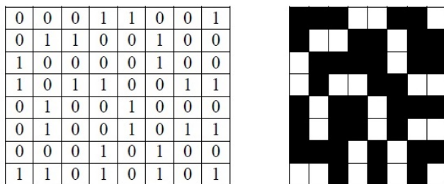
Fig. 3 An exactly-1-4-adjacent binary matrix
