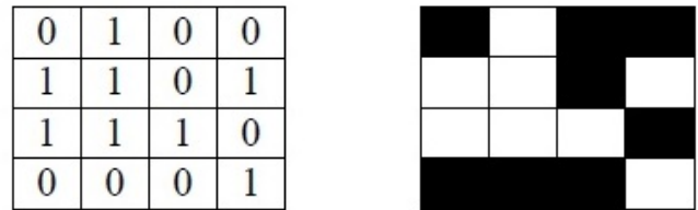
Fig. 1 Two representations of the same binary matrix
