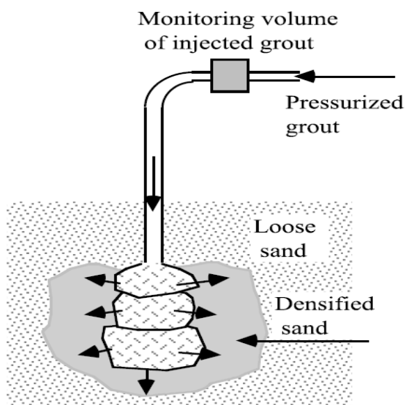
Fig. 1 Compaction Grouting Procedure [9]
