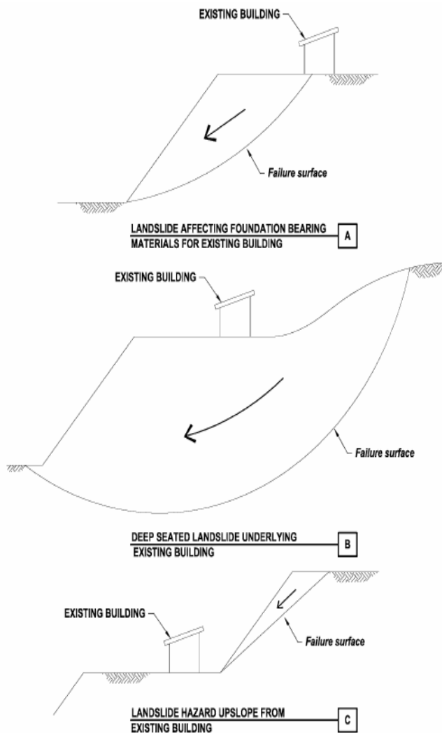
Fig. 4 Landslide Hazards [1]
