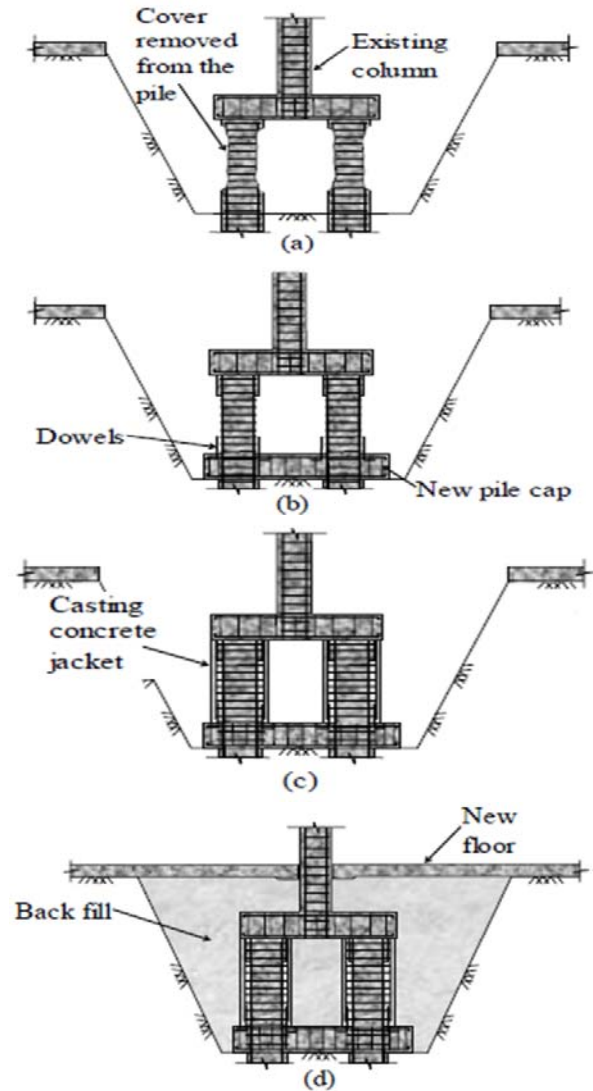
Fig. 8 Strengthening of the Existing Piles [3]
