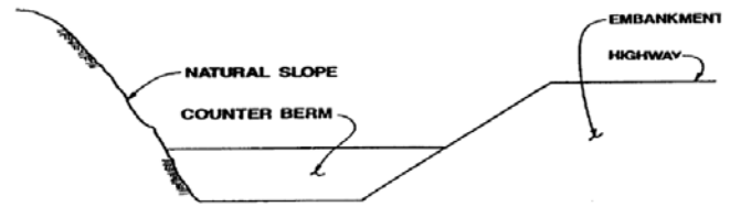
Fig. 6 Using Counterberms at the Slope Toe [10]
